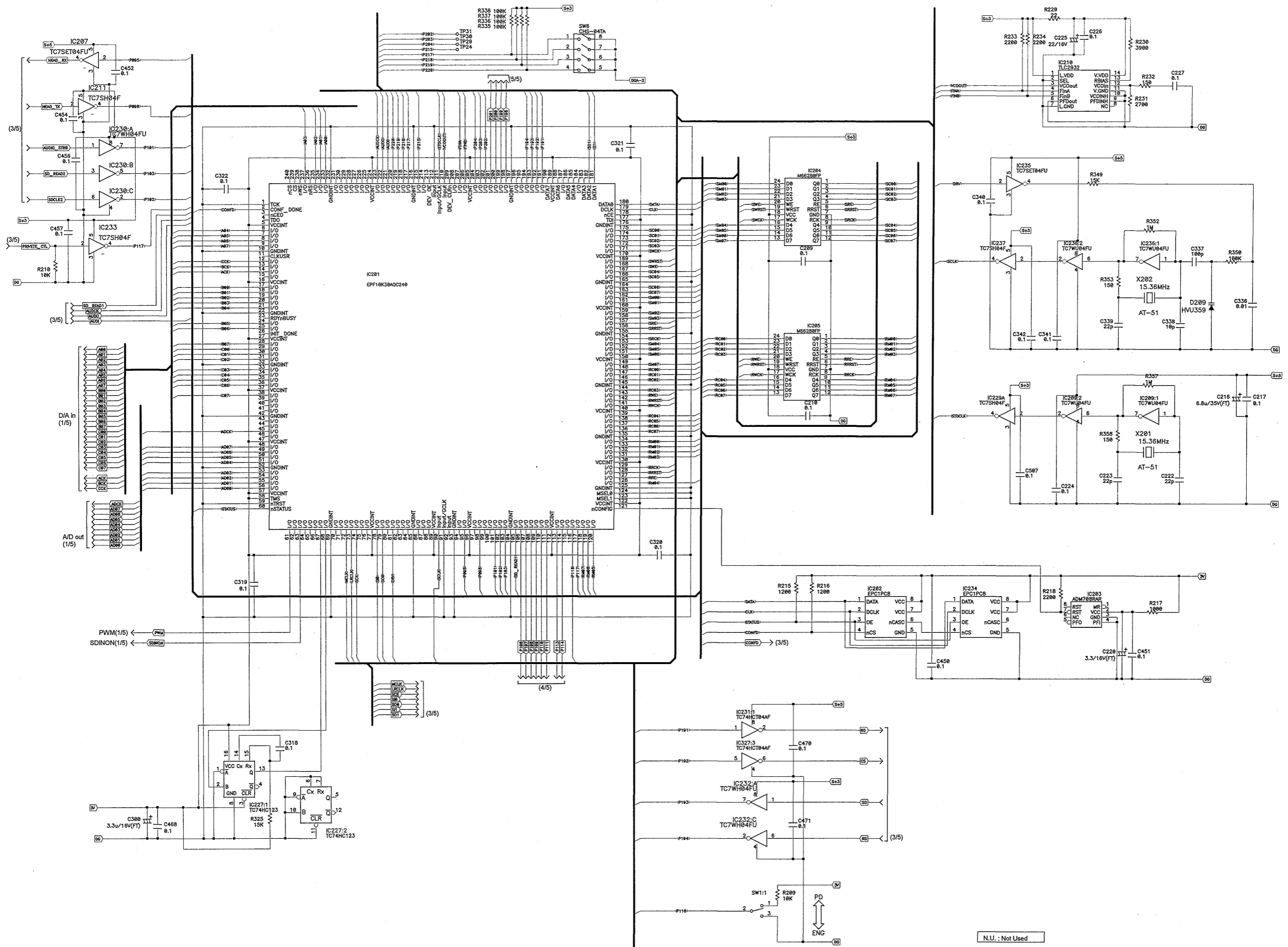
TU-Z3A TU-PWR/INCOM UNIT(INCOM) SCHEMATIC DIAGRAM(2/5)
